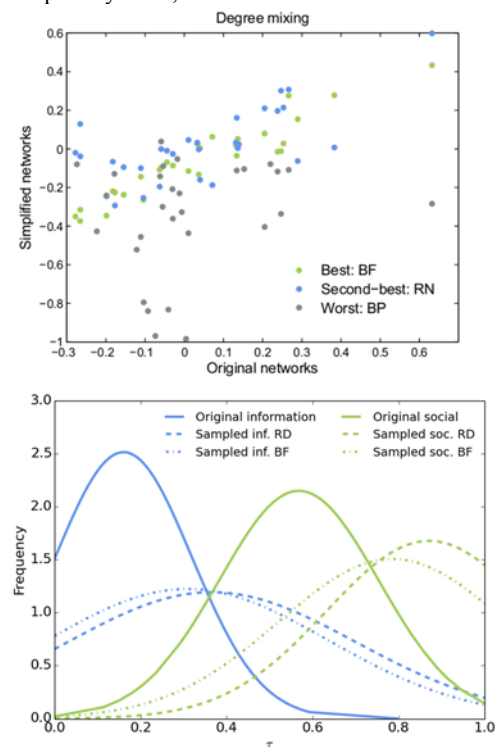
Figure 1: (above) The relationship between the degree mixing of original and simplified networks. The breadth-first sampling proved as the best method. (below) The distribution of group parameter \tau (i.e., \tau=1 denotes communities, \tau=0 modules and 0 < \tau < 1 mixtures). Sampled networks are characterized by larger number of communities and mixtures than original networks in social and information networks, respectively.
